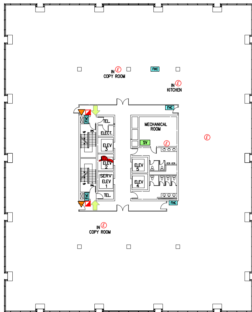
9th FLOOR
