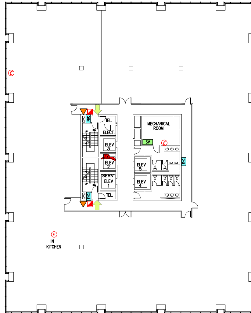
2nd FLOOR
